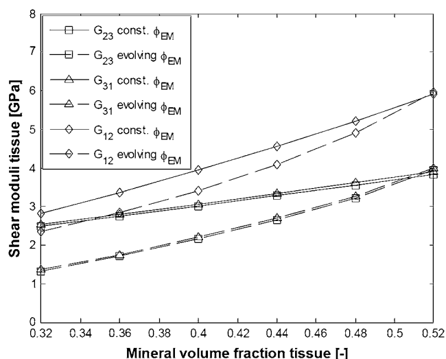
FIGURE 9 Shear moduli of bundles of aligned fibrils with EF mineralization (parameters from Table 1). (Solid lines, constant \phi_{EM} ; dashed lines, evolving \phi_{EM} ; squares, G_{23} ; triangles, G_{31} ; diamonds, G_{12} .)
